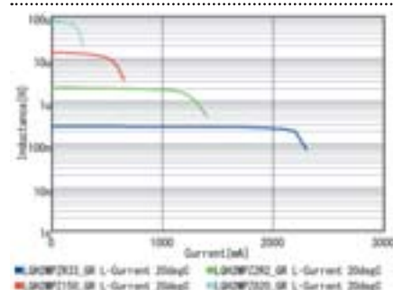
Inductance-Current Characteristics (Typ.)
