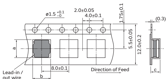
c: Depth of Cavity
